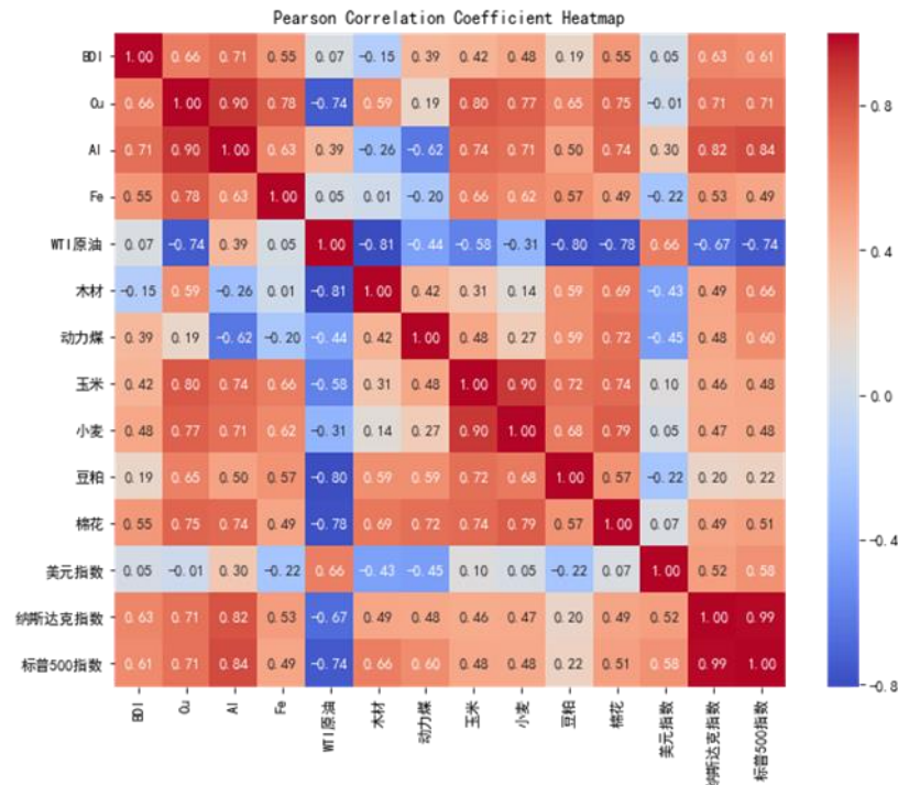
Figure 4-1 Heatmap of Influencing Factors
