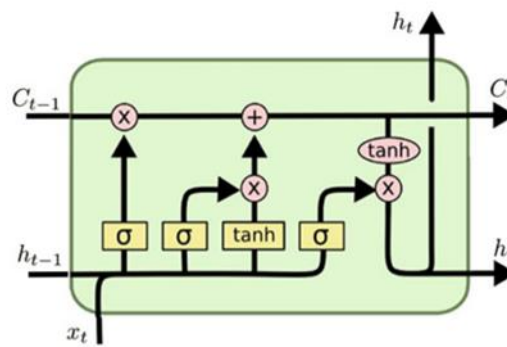
Figure 4-2 Gate Control Mechanisms in the LSTM Neural Network Model
