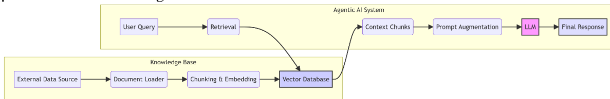
Figure 3. Retrieval-Augmented Generation (RAG) Memory Architecture
