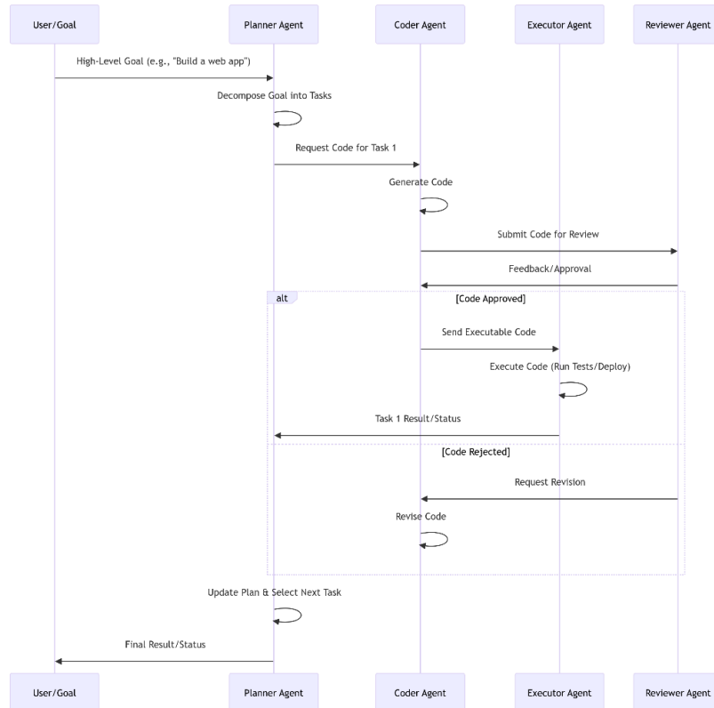
Figure 6. Multi-Agent System Collaborative Workflow
