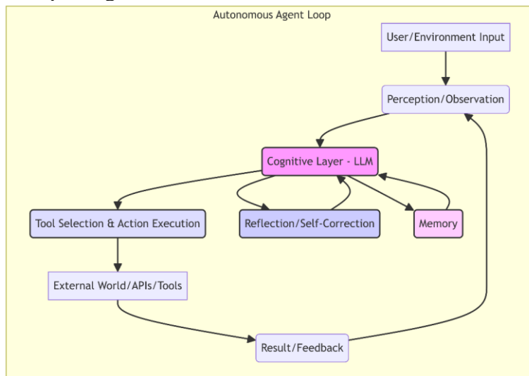
Figure 2. Agentic AI Autonomous Loop Architecture
