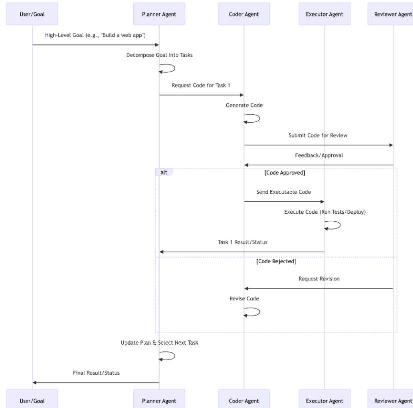
Figure 4. Multi-Agent System Collaborative Workflow
