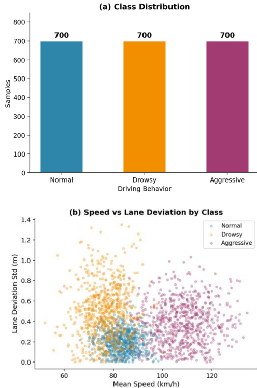
Figure 1. (a) Class distribution of the driving behavior dataset. (b) Scatter plot of speed mean vs. lane deviation std by class, illustrating inter-class overlap.
